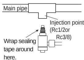
A-3. FTCT/6TCT type
